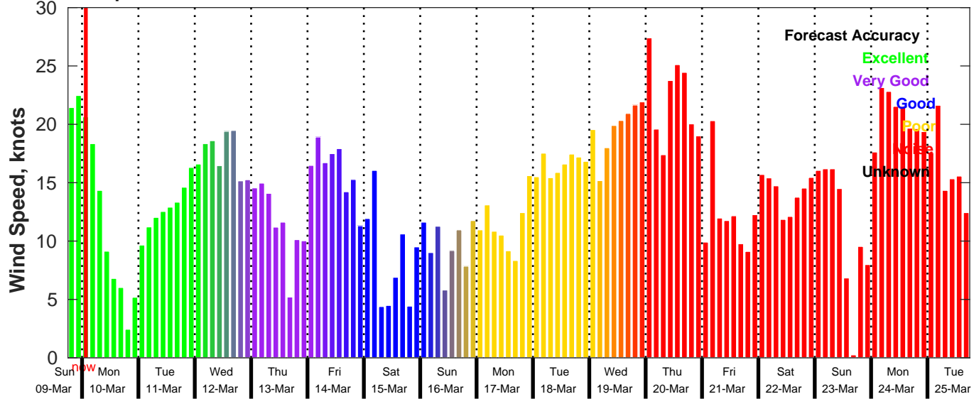
GFS Wind Speed Forecast for NDBC 42019 from 09-Mar-2025 18:00:00 to 25-Mar-2025 18:00:00
