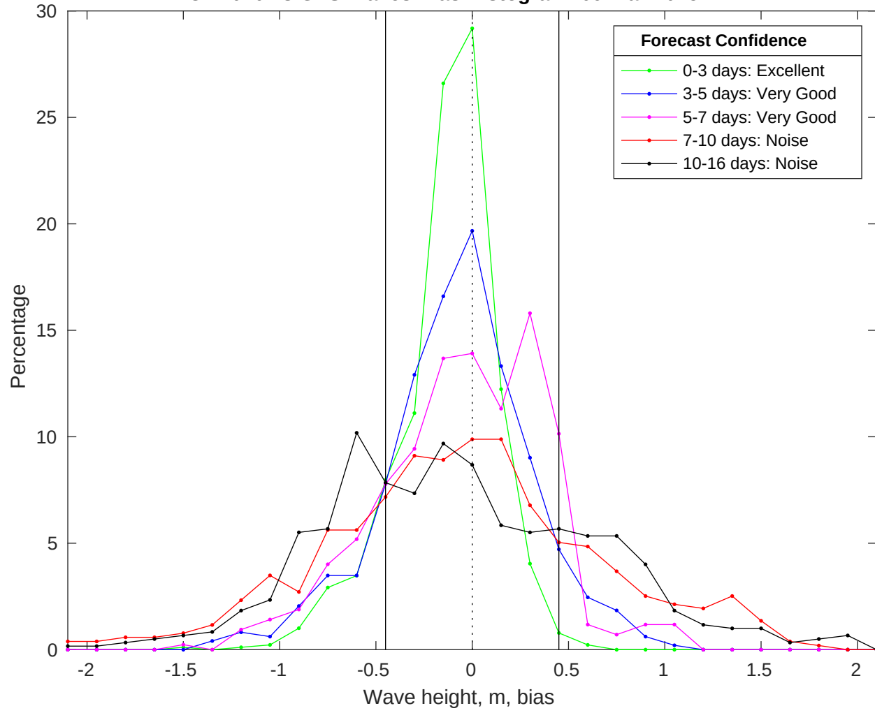
NDBC 42020 vs GFS Waves Bias Histogram: 09-Mar-2025
