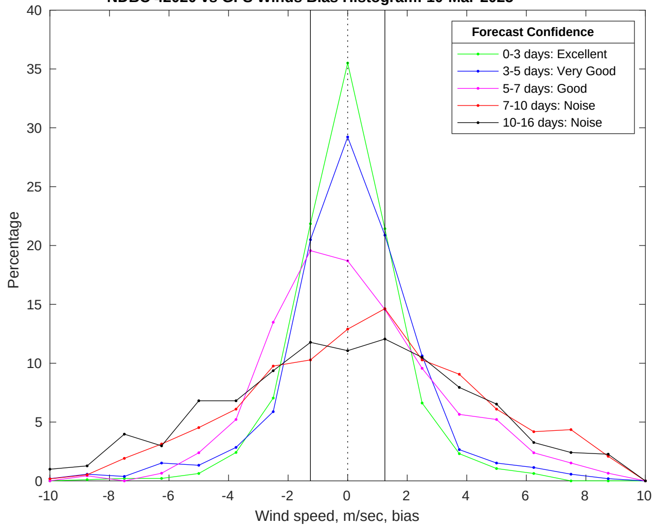
NDBC 42020 vs GFS Winds Bias Histogram: 10-Mar-2025
