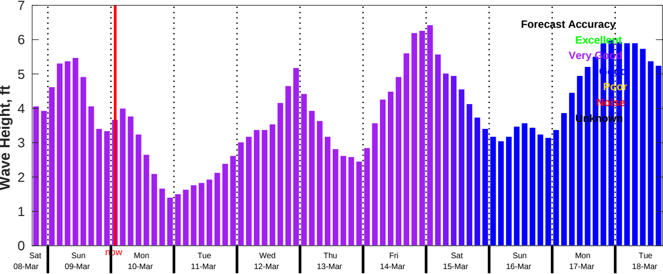
CMEMS Wave Forecast for NDBC 42020 from 08-Mar-2025 18:00:00 to 18-Mar-2025 18:00:00
