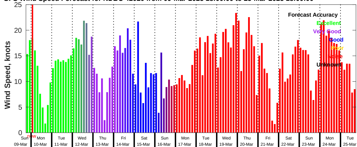
GFS Wind Speed Forecast for NDBC 42020 from 09-Mar-2025 18:00:00 to 25-Mar-2025 18:00:00
