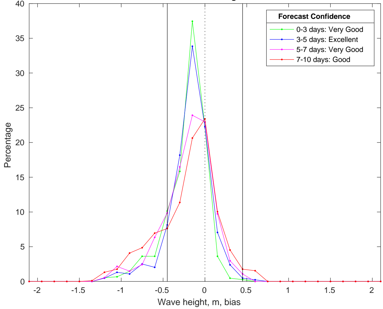
NDBC 42035 vs CMEMS Waves Bias Histogram: 10-Mar-2025
