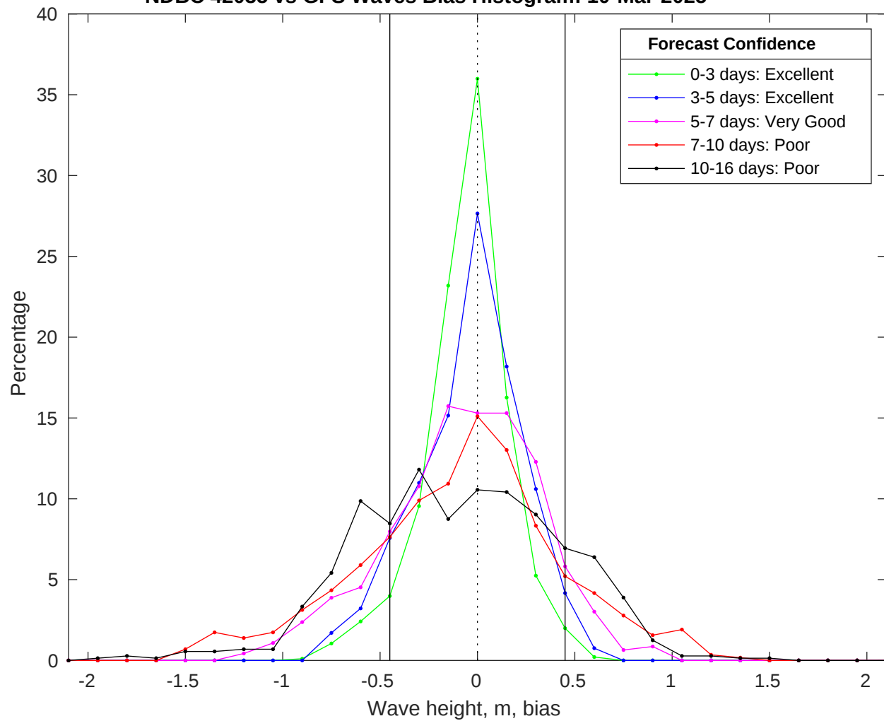
NDBC 42035 vs GFS Waves Bias Histogram: 10-Mar-2025
