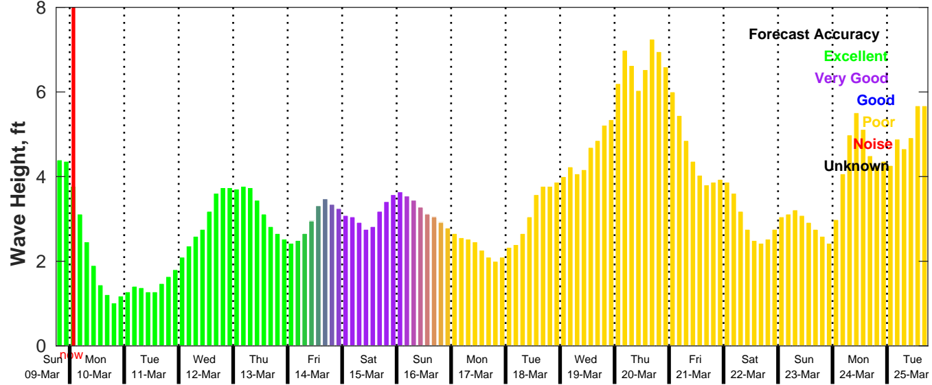
GFS Wave Forecast for NDBC 42035 from 09-Mar-2025 18:00:00 to 25-Mar-2025 18:00:00
