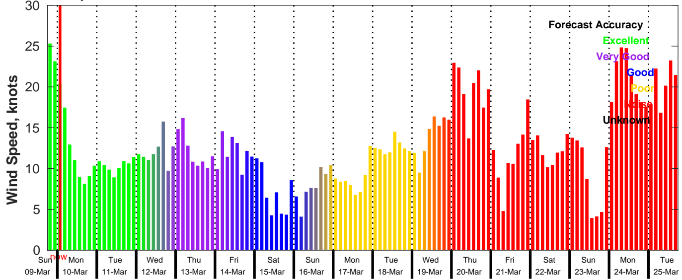
GFS Wind Speed Forecast for NDBC 42035 from 09-Mar-2025 18:00:00 to 25-Mar-2025 18:00:00
