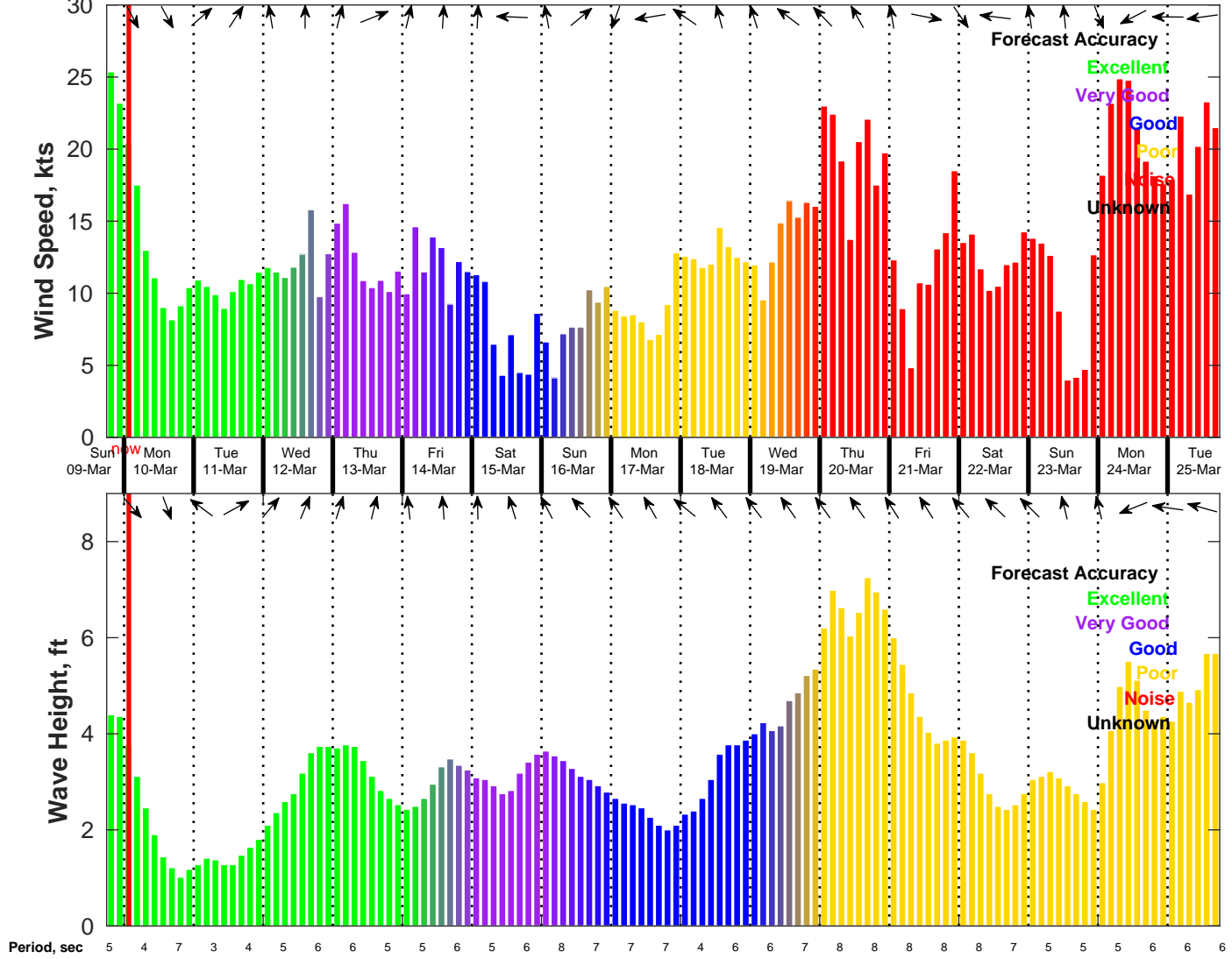
Wind & Wave Forecast for NDBC 42035 from 09-Mar-2025 18:00:00 to 25-Mar-2025 18:00:00
