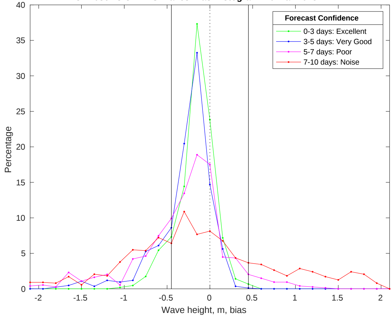
NDBC 42036 vs CMEMS Waves Bias Histogram: 10-Mar-2025
