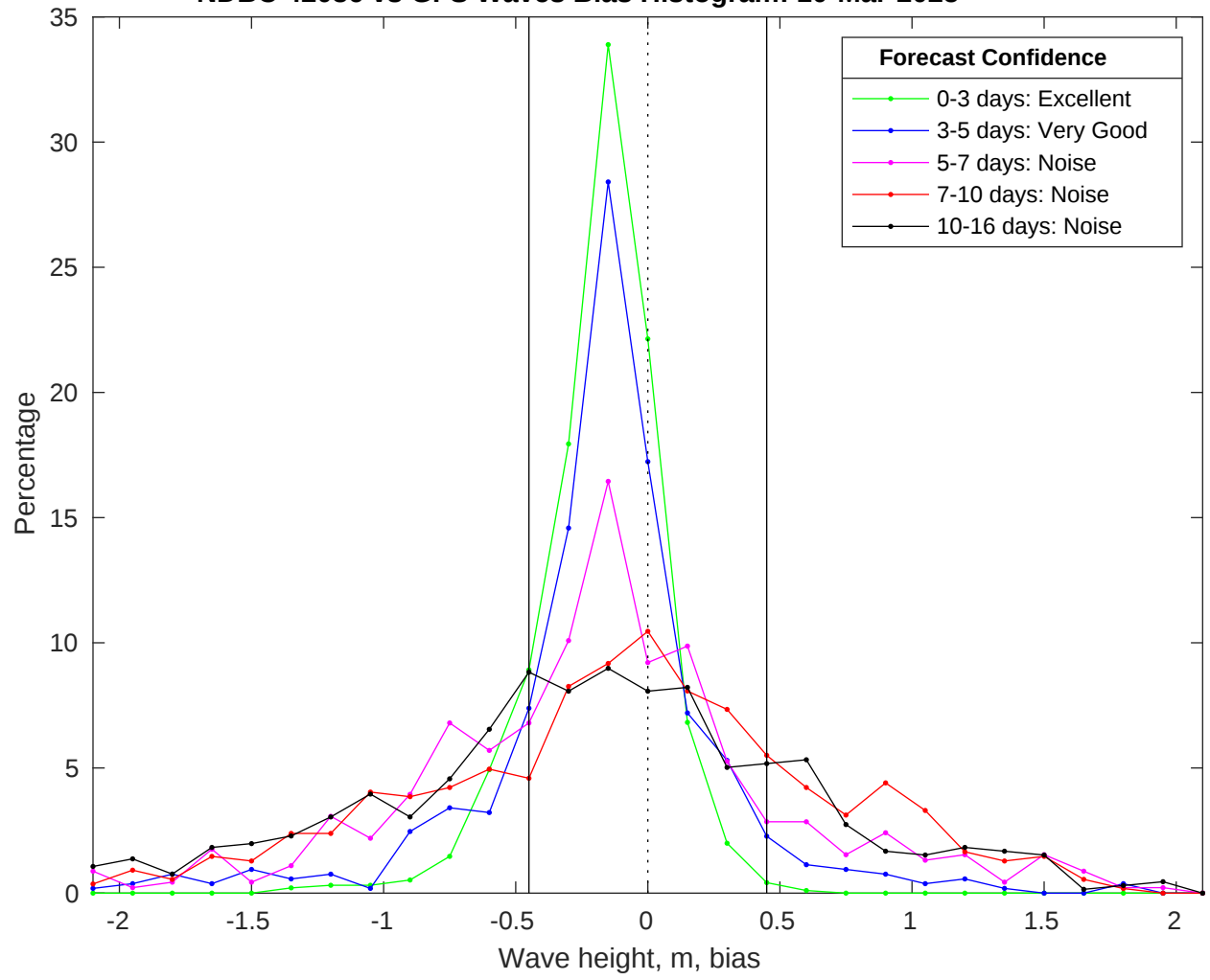
NDBC 42036 vs GFS Waves Bias Histogram: 10-Mar-2025
