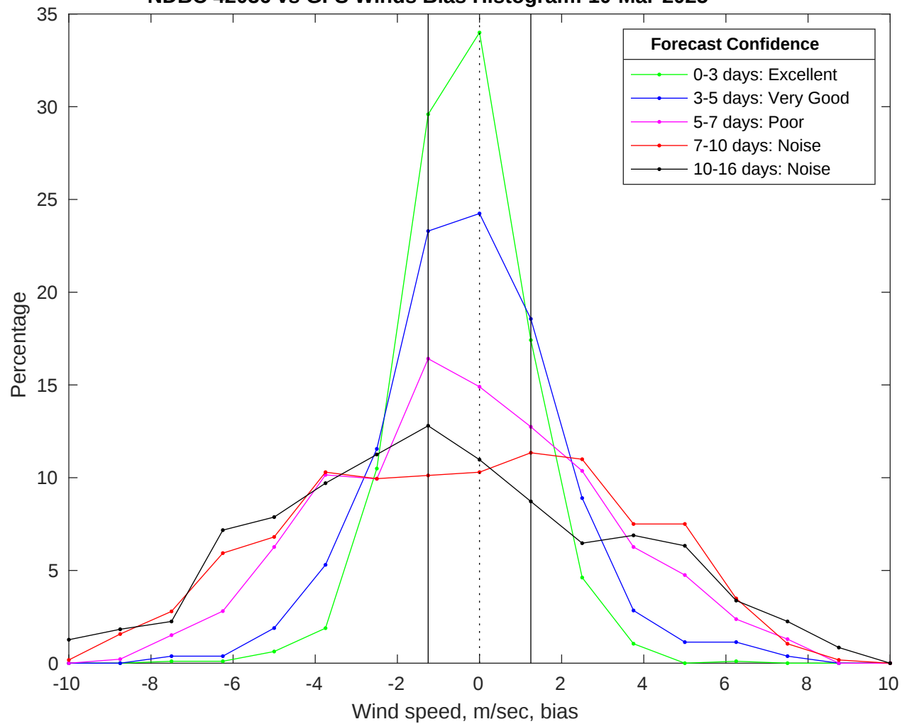
NDBC 42036 vs GFS Winds Bias Histogram: 10-Mar-2025
