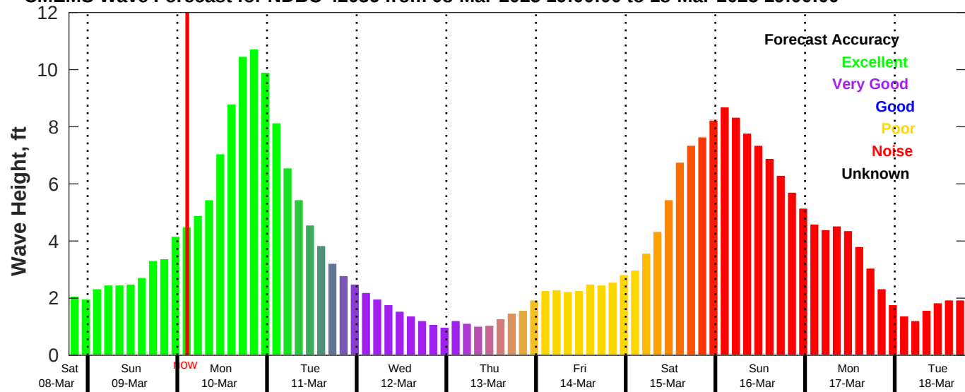
CMEMS Wave Forecast for NDBC 42036 from 08-Mar-2025 19:00:00 to 18-Mar-2025 19:00:00
