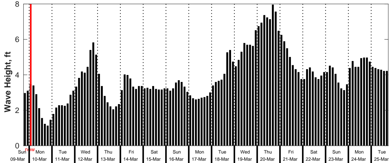
GFS Wave Forecast for NDBC 42092 from 09-Mar-2025 18:00:00 to 25-Mar-2025 18:00:00
