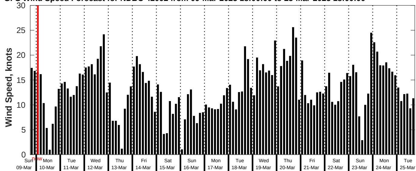
GFS Wind Speed Forecast for NDBC 42092 from 09-Mar-2025 18:00:00 to 25-Mar-2025 18:00:00
