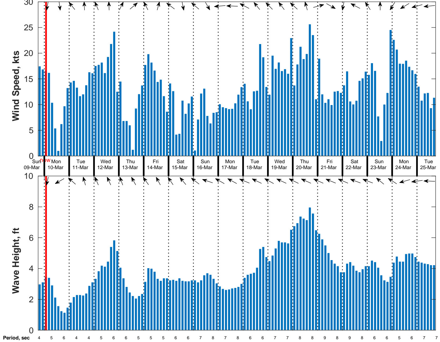
Wind & Wave Forecast for NDBC 42092 from 09-Mar-2025 18:00:00 to 25-Mar-2025 18:00:00
