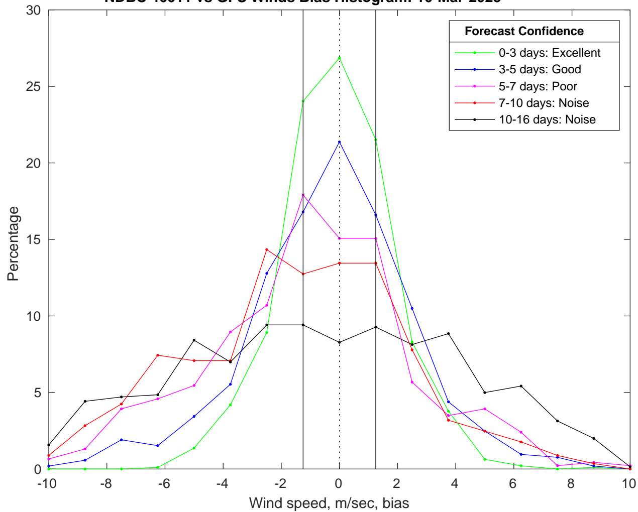
NDBC 46011 vs GFS Winds Bias Histogram: 10-Mar-2025
