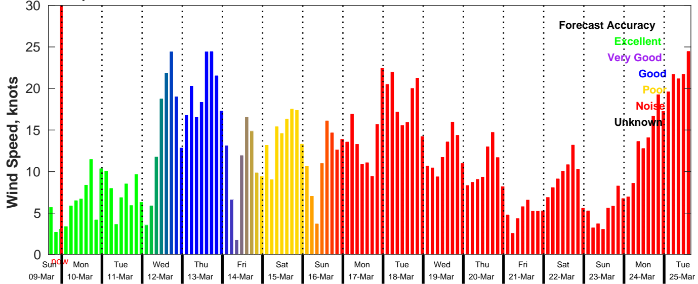
GFS Wind Speed Forecast for NDBC 46011 from 09-Mar-2025 16:00:00 to 25-Mar-2025 16:00:00
