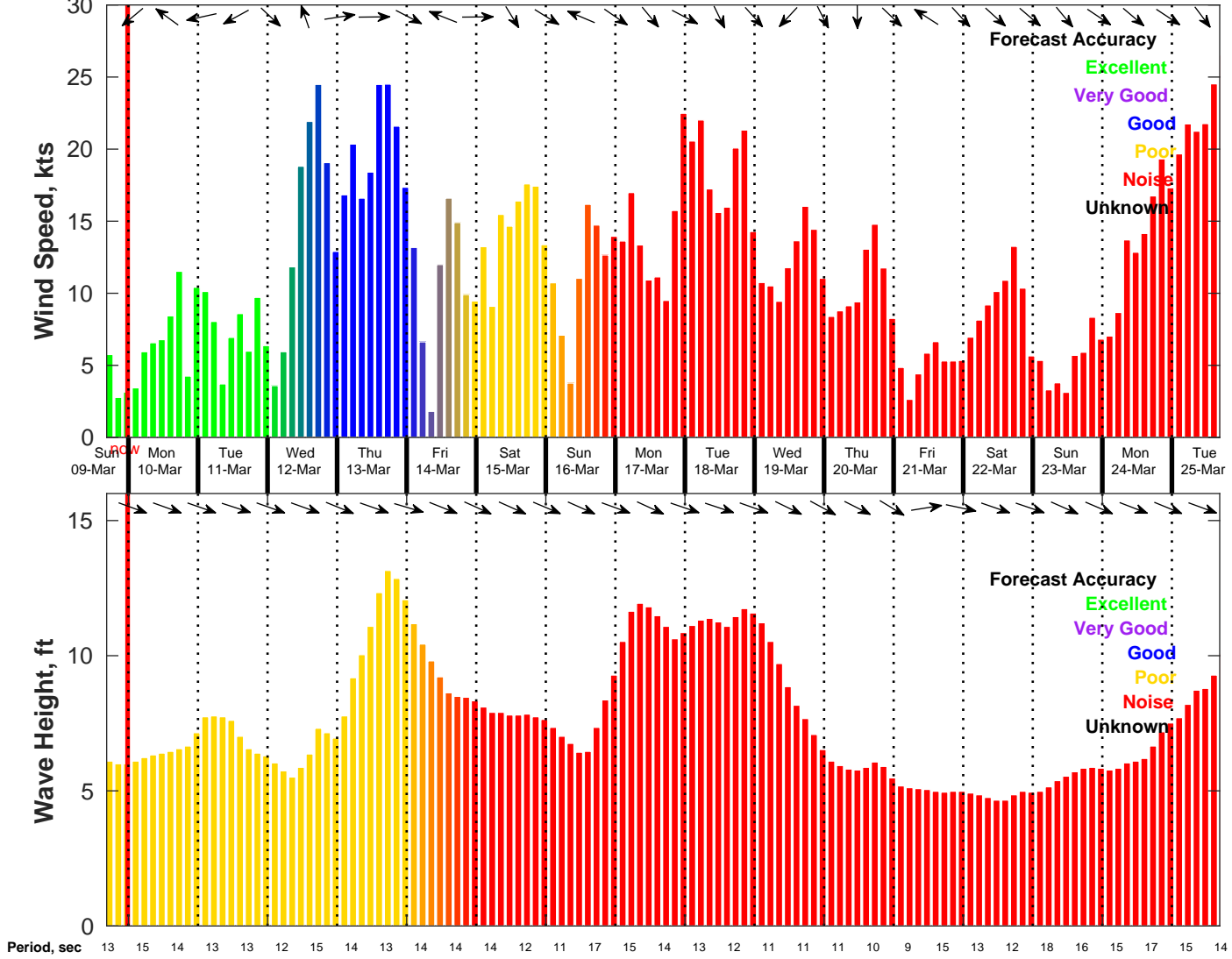
Wind & Wave Forecast for NDBC 46011 from 09-Mar-2025 16:00:00 to 25-Mar-2025 16:00:00
