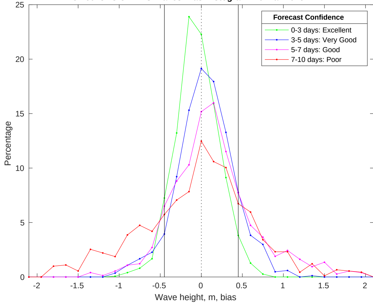
NDBC 46028 vs CMEMS Waves Bias Histogram: 10-Mar-2025
