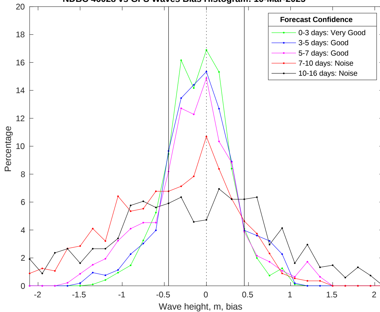
NDBC 46028 vs GFS Waves Bias Histogram: 10-Mar-2025
