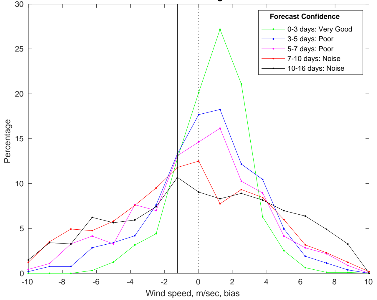
NDBC 46028 vs GFS Winds Bias Histogram: 10-Mar-2025
