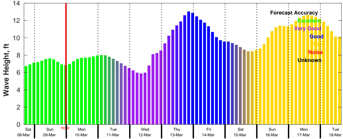
CMEMS Wave Forecast for NDBC 46028 from 08-Mar-2025 16:00:00 to 18-Mar-2025 16:00:00
