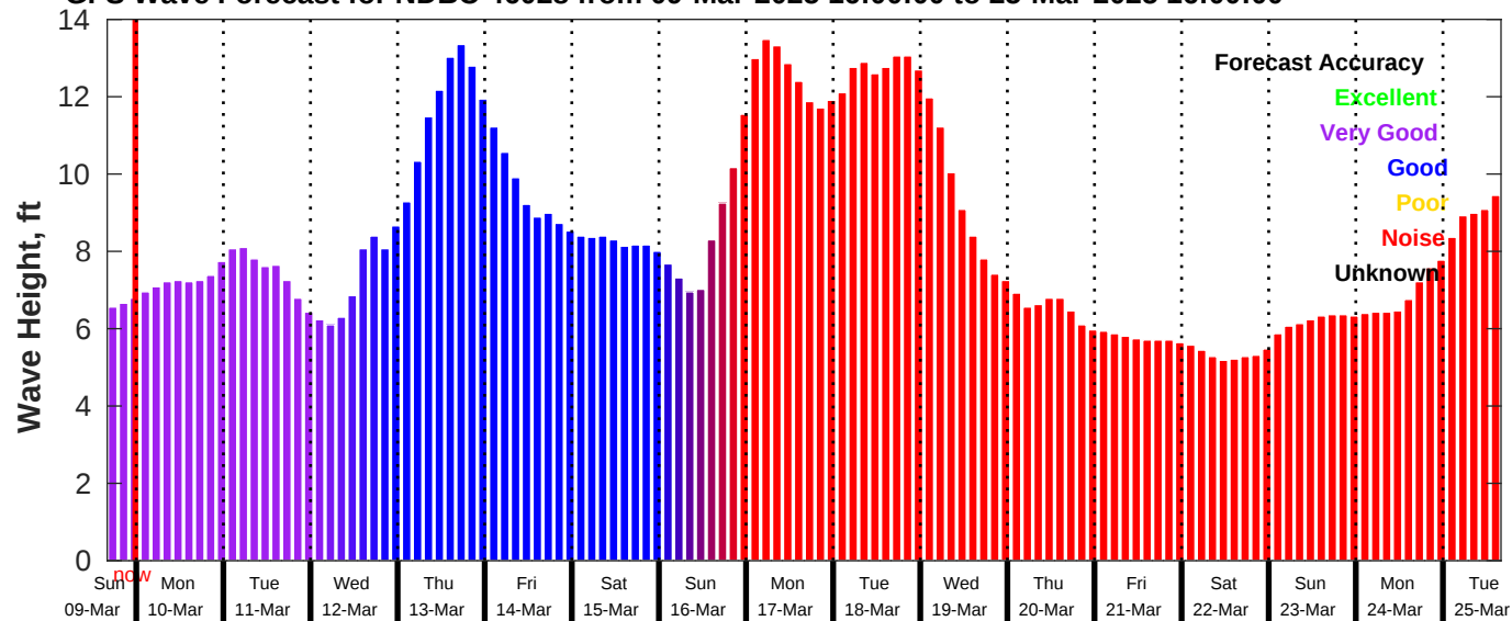
GFS Wave Forecast for NDBC 46028 from 09-Mar-2025 16:00:00 to 25-Mar-2025 16:00:00
