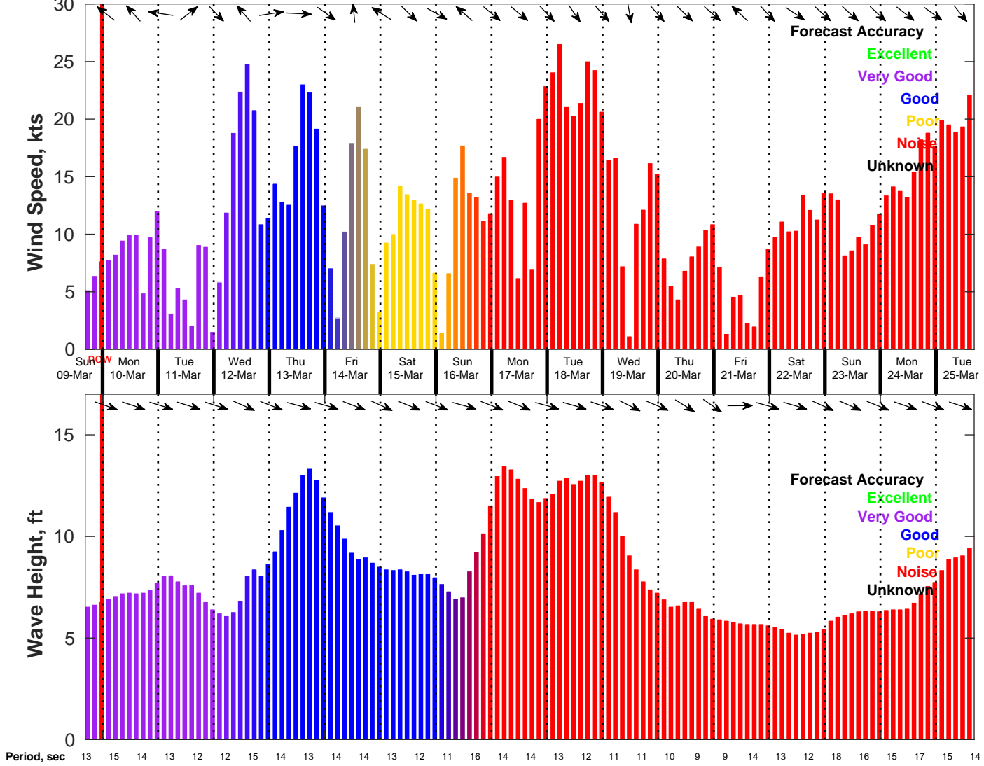
Wind & Wave Forecast for NDBC 46028 from 09-Mar-2025 16:00:00 to 25-Mar-2025 16:00:00
