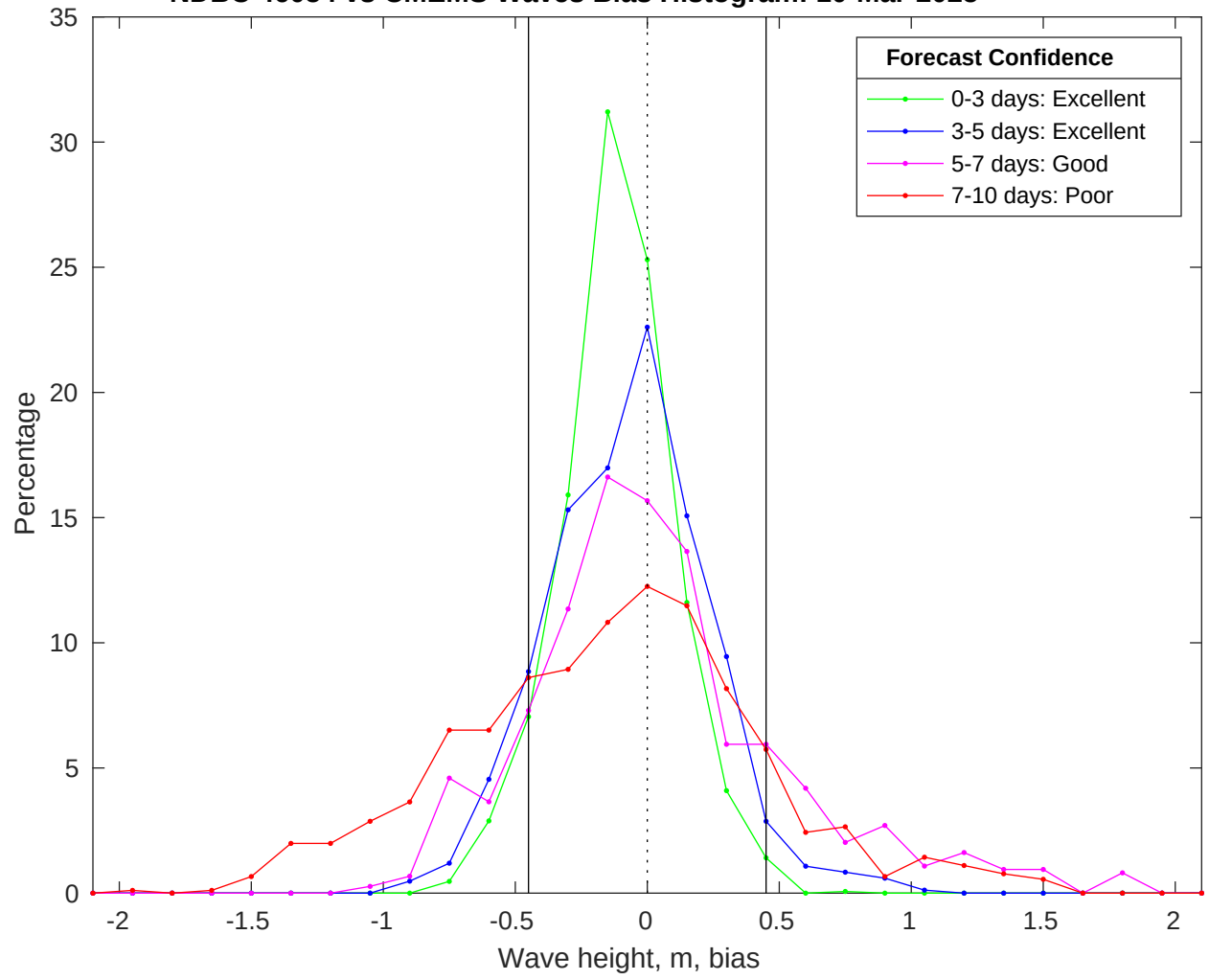
NDBC 46054 vs CMEMS Waves Bias Histogram: 10-Mar-2025
