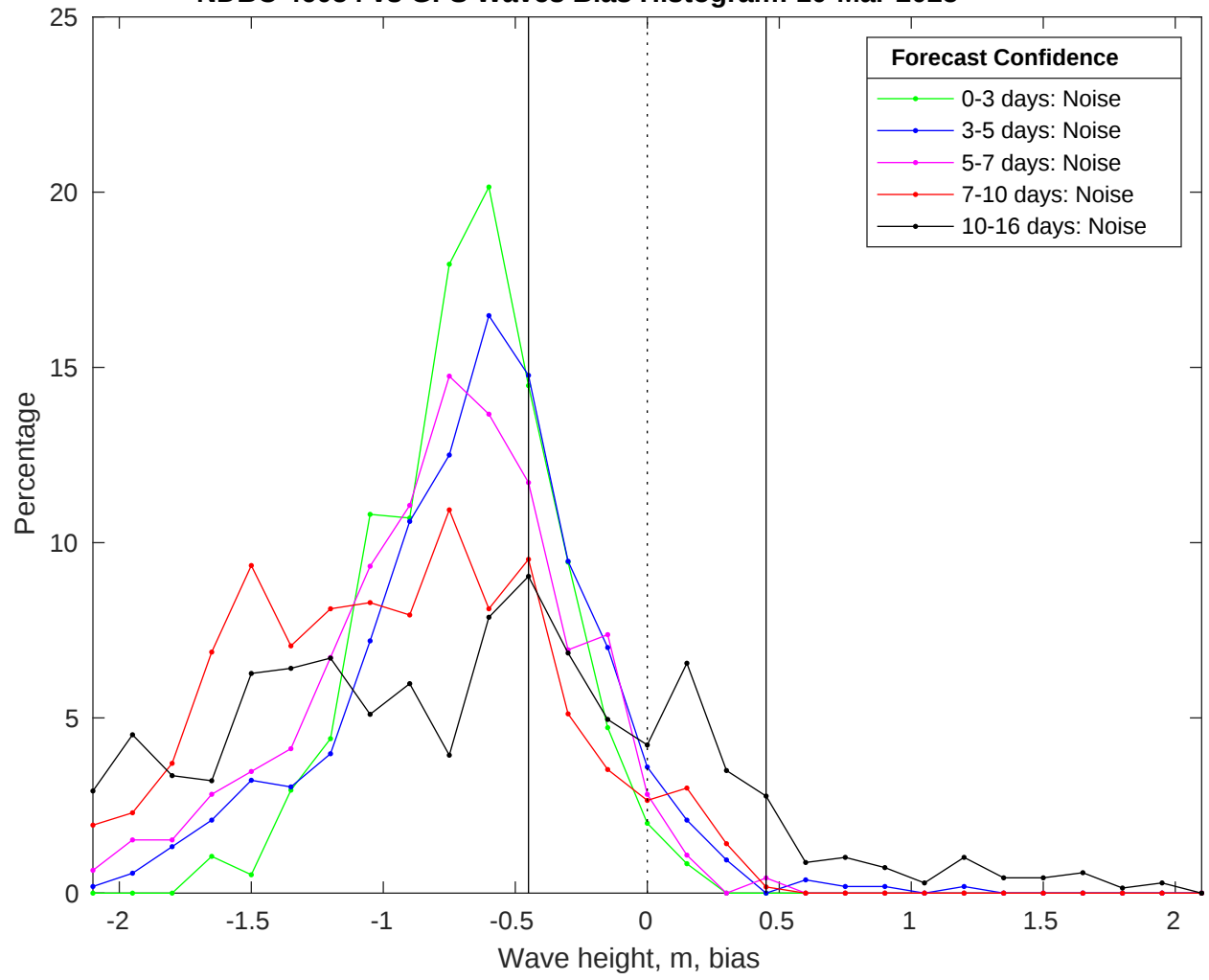
NDBC 46054 vs GFS Waves Bias Histogram: 10-Mar-2025
