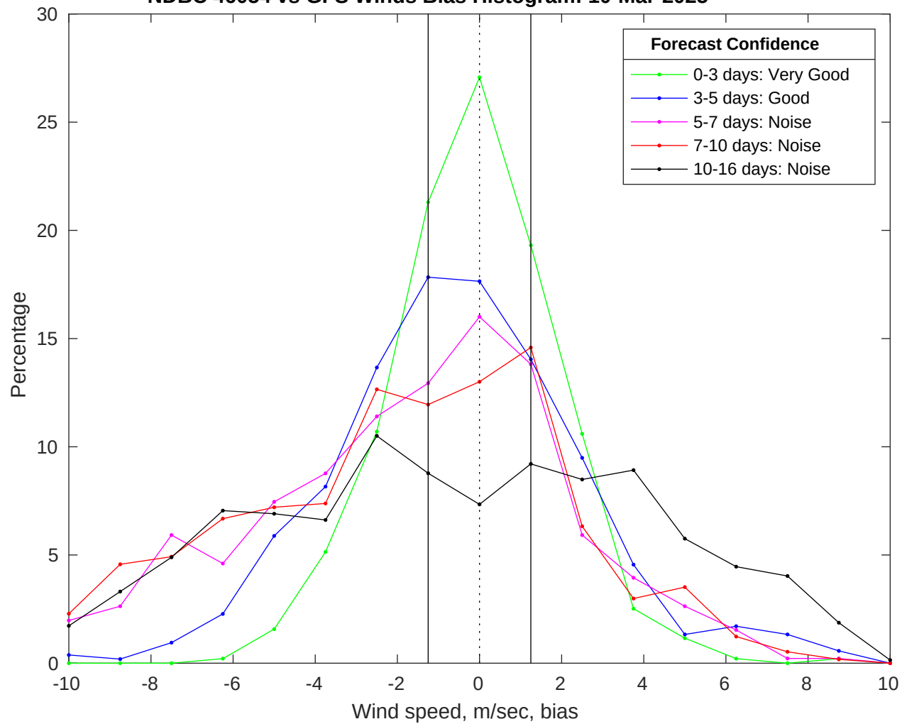
NDBC 46054 vs GFS Winds Bias Histogram: 10-Mar-2025
