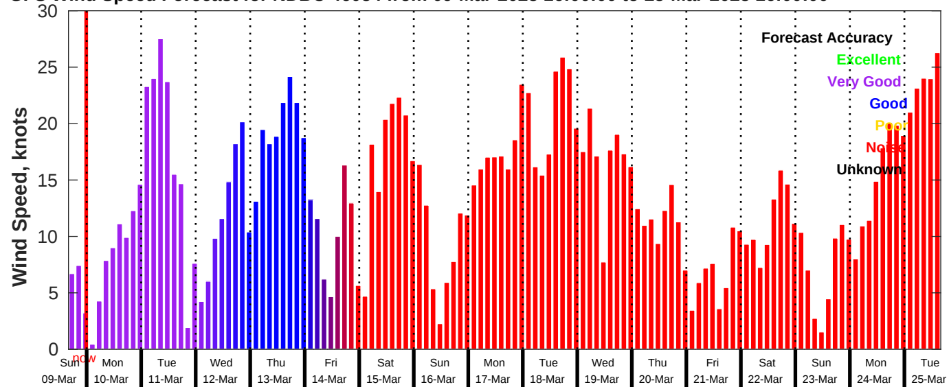
GFS Wind Speed Forecast for NDBC 46054 from 09-Mar-2025 16:00:00 to 25-Mar-2025 16:00:00
