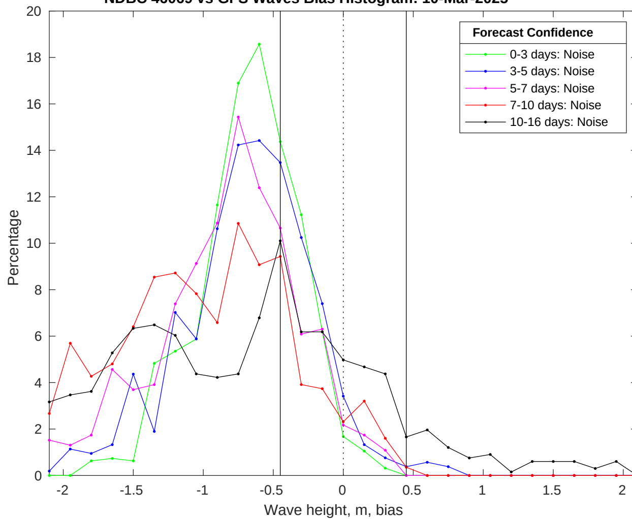
NDBC 46069 vs GFS Waves Bias Histogram: 10-Mar-2025
