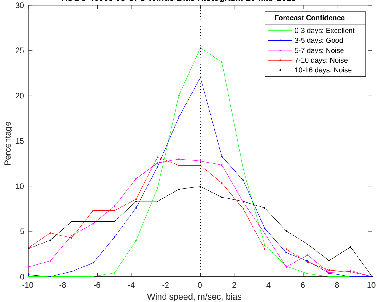
NDBC 46069 vs GFS Winds Bias Histogram: 10-Mar-2025
