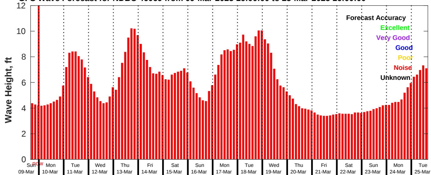
GFS Wave Forecast for NDBC 46069 from 09-Mar-2025 16:00:00 to 25-Mar-2025 16:00:00
