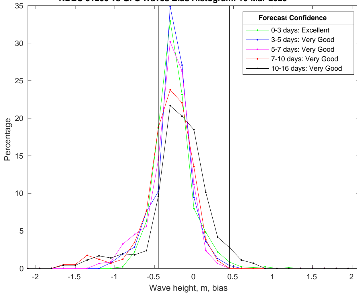
NDBC 51209 vs GFS Waves Bias Histogram: 10-Mar-2025
