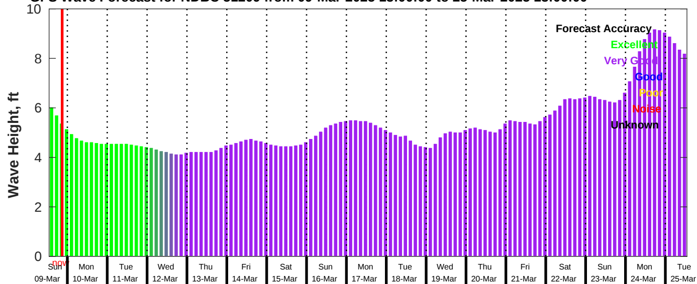
GFS Wave Forecast for NDBC 51209 from 09-Mar-2025 13:00:00 to 25-Mar-2025 13:00:00
