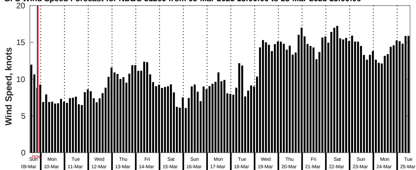
GFS Wind Speed Forecast for NDBC 51209 from 09-Mar-2025 13:00:00 to 25-Mar-2025 13:00:00
