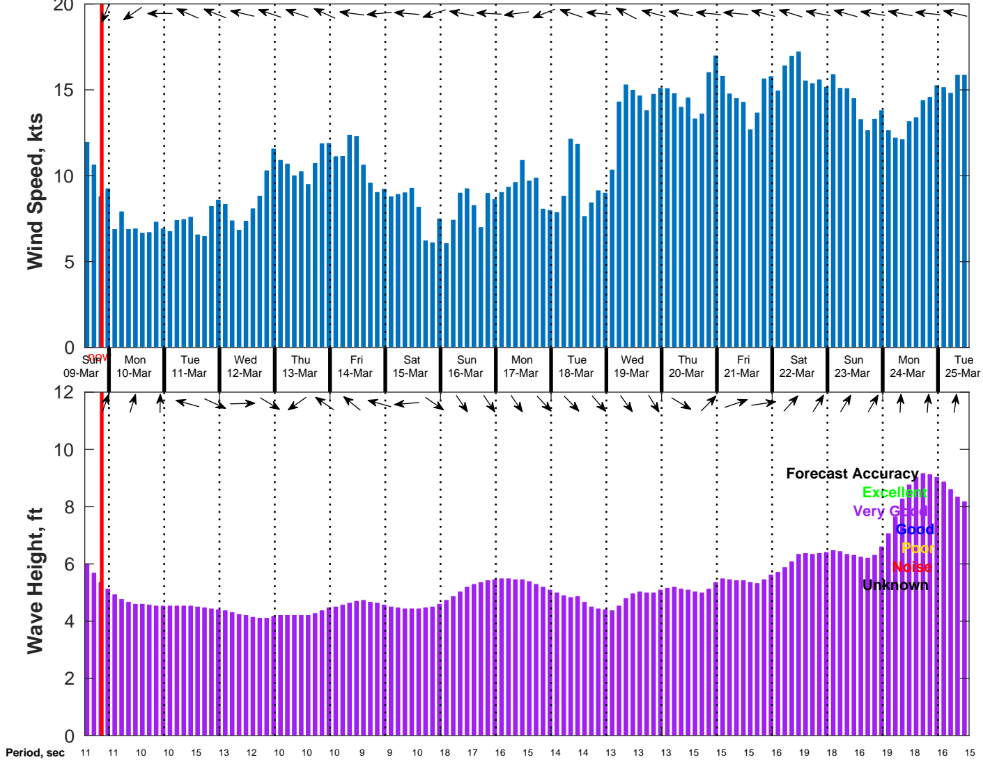
Wind & Wave Forecast for NDBC 51209 from 09-Mar-2025 13:00:00 to 25-Mar-2025 13:00:00
