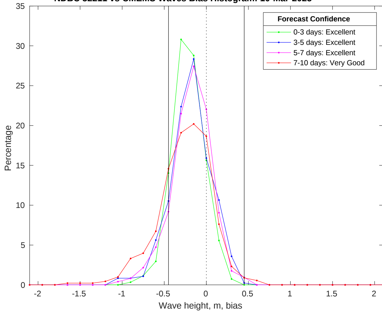
NDBC 52211 vs CMEMS Waves Bias Histogram: 10-Mar-2025
