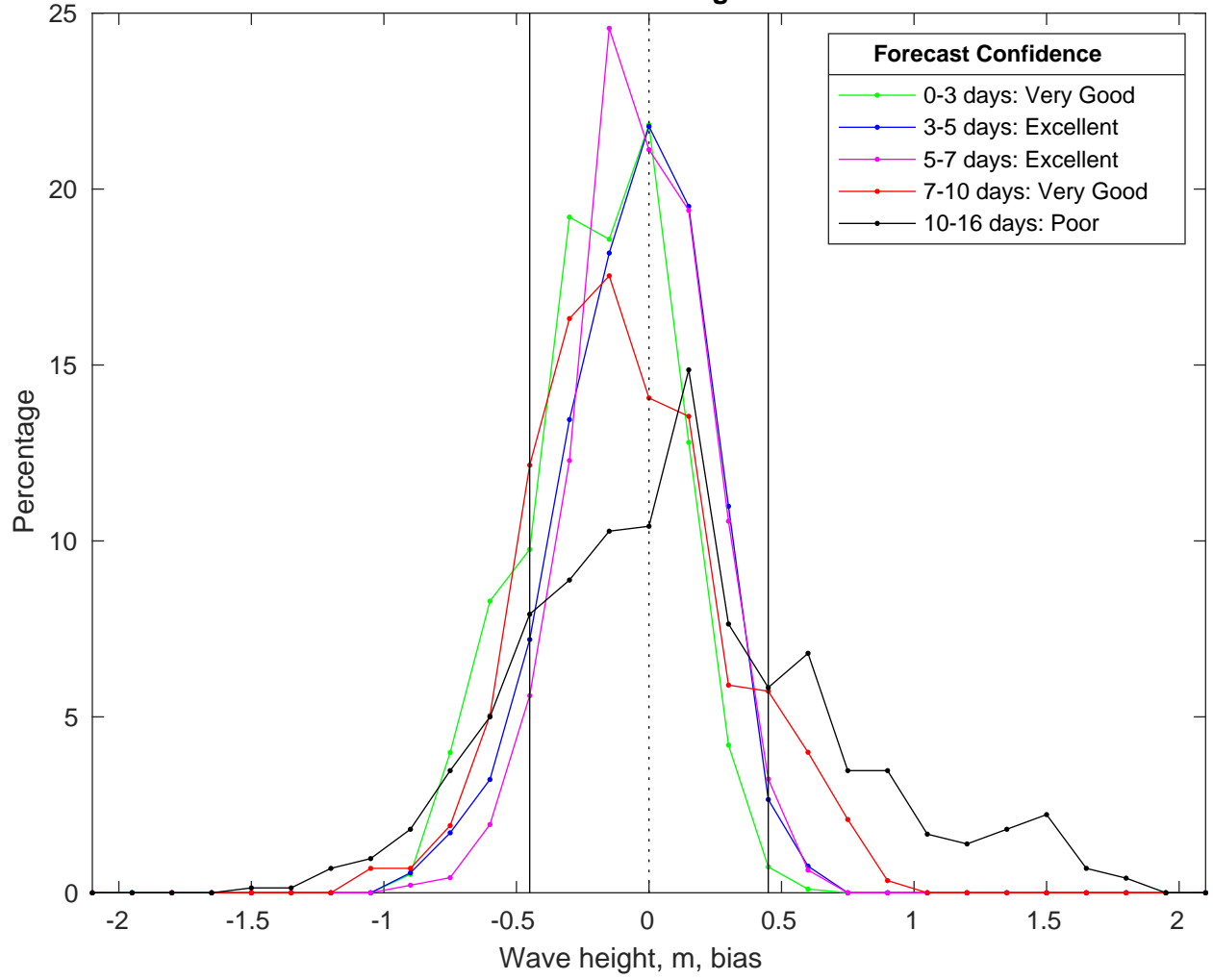
NDBC 52211 vs GFS Waves Bias Histogram: 10-Mar-2025
