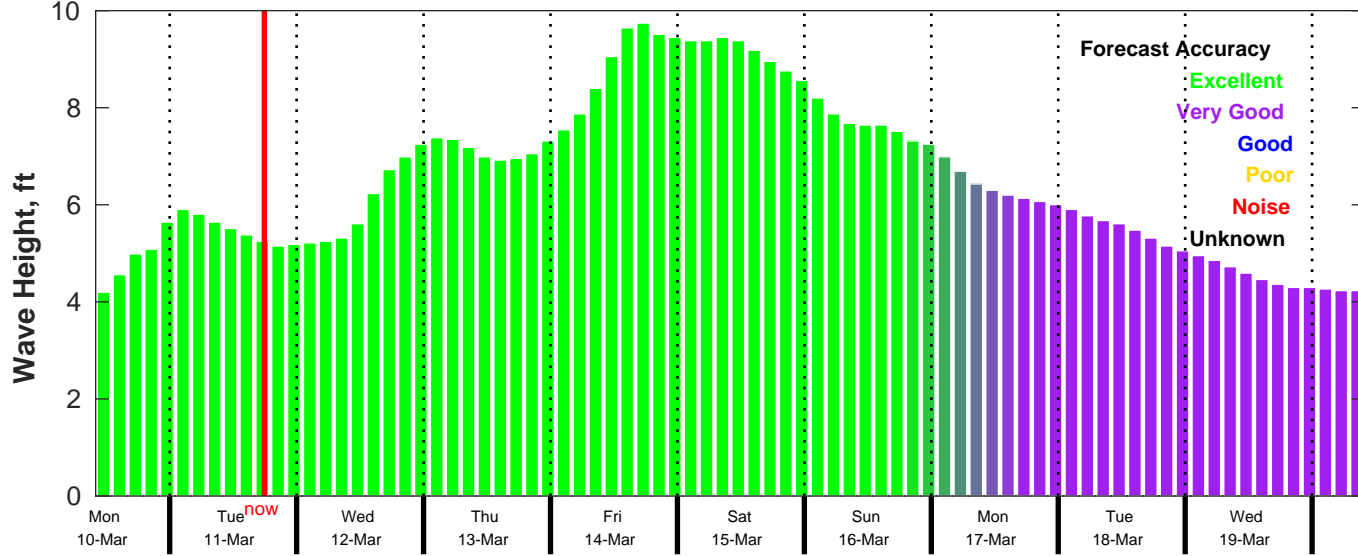
CMEMS Wave Forecast for NDBC 52211 from 09-Mar-2025 10:00:00 to 19-Mar-2025 10:00:00
