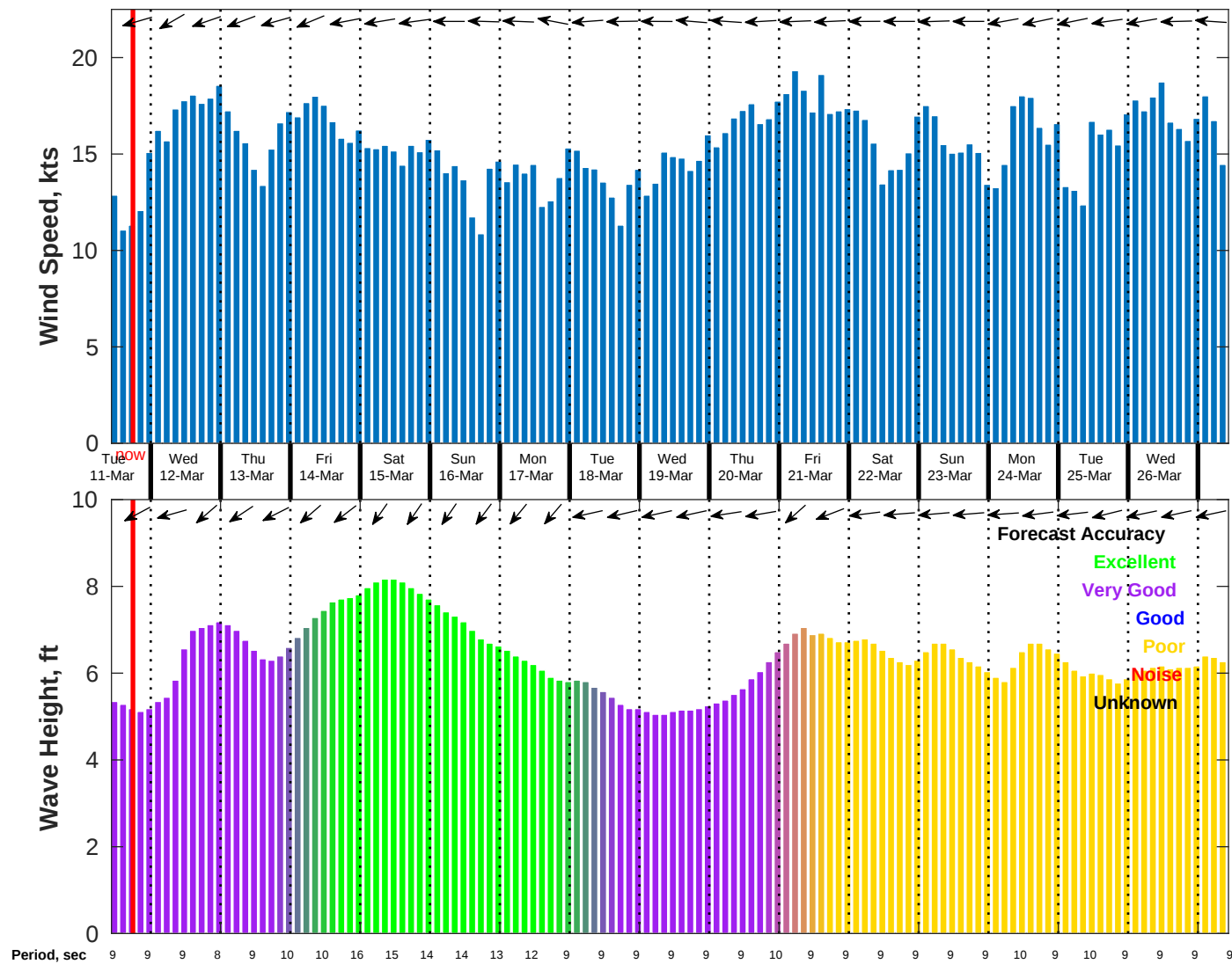
Wind & Wave Forecast for NDBC 52211 from 10-Mar-2025 10:00:00 to 26-Mar-2025 10:00:00
