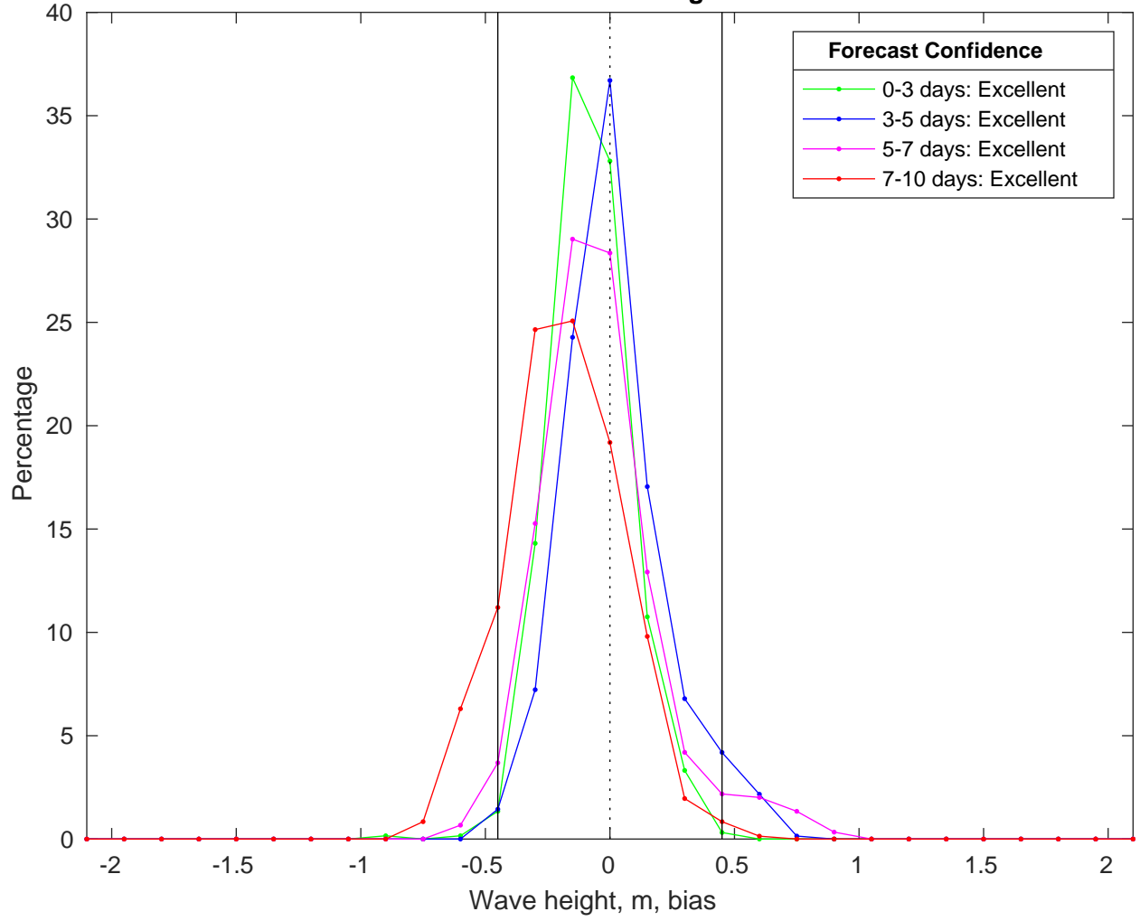
NDBC 52212 vs CMEMS Waves Bias Histogram: 10-Mar-2025
