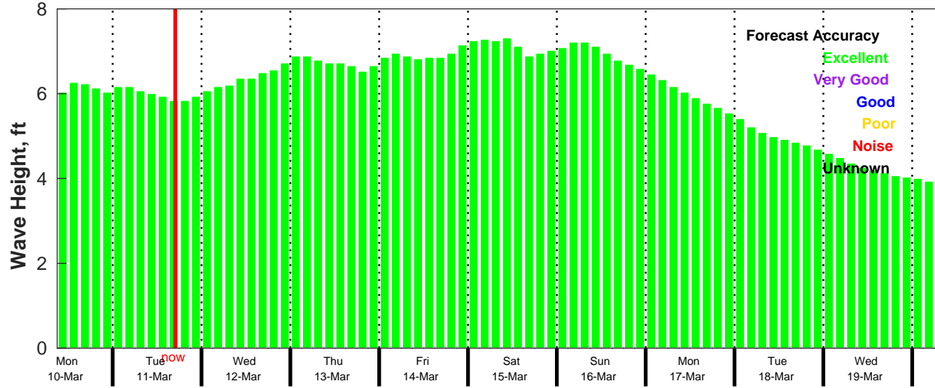
CMEMS Wave Forecast for NDBC 52212 from 09-Mar-2025 09:00:00 to 19-Mar-2025 09:00:00
