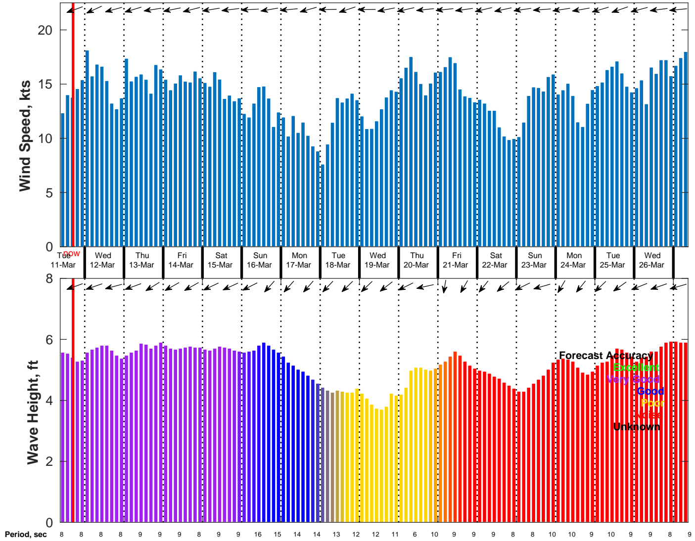
Wind & Wave Forecast for NDBC 52212 from 10-Mar-2025 09:00:00 to 26-Mar-2025 09:00:00
