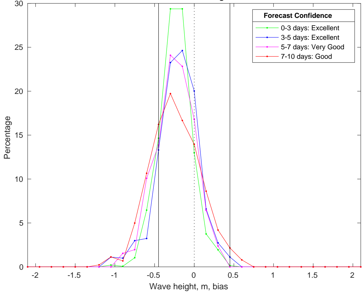
NDBC 52213 vs CMEMS Waves Bias Histogram: 10-Mar-2025
