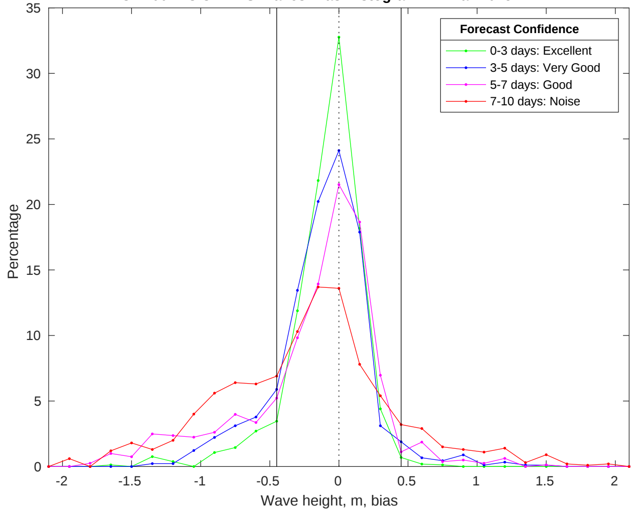
NDBC 41004 vs CMEMS Waves Bias Histogram: 11-Mar-2025
