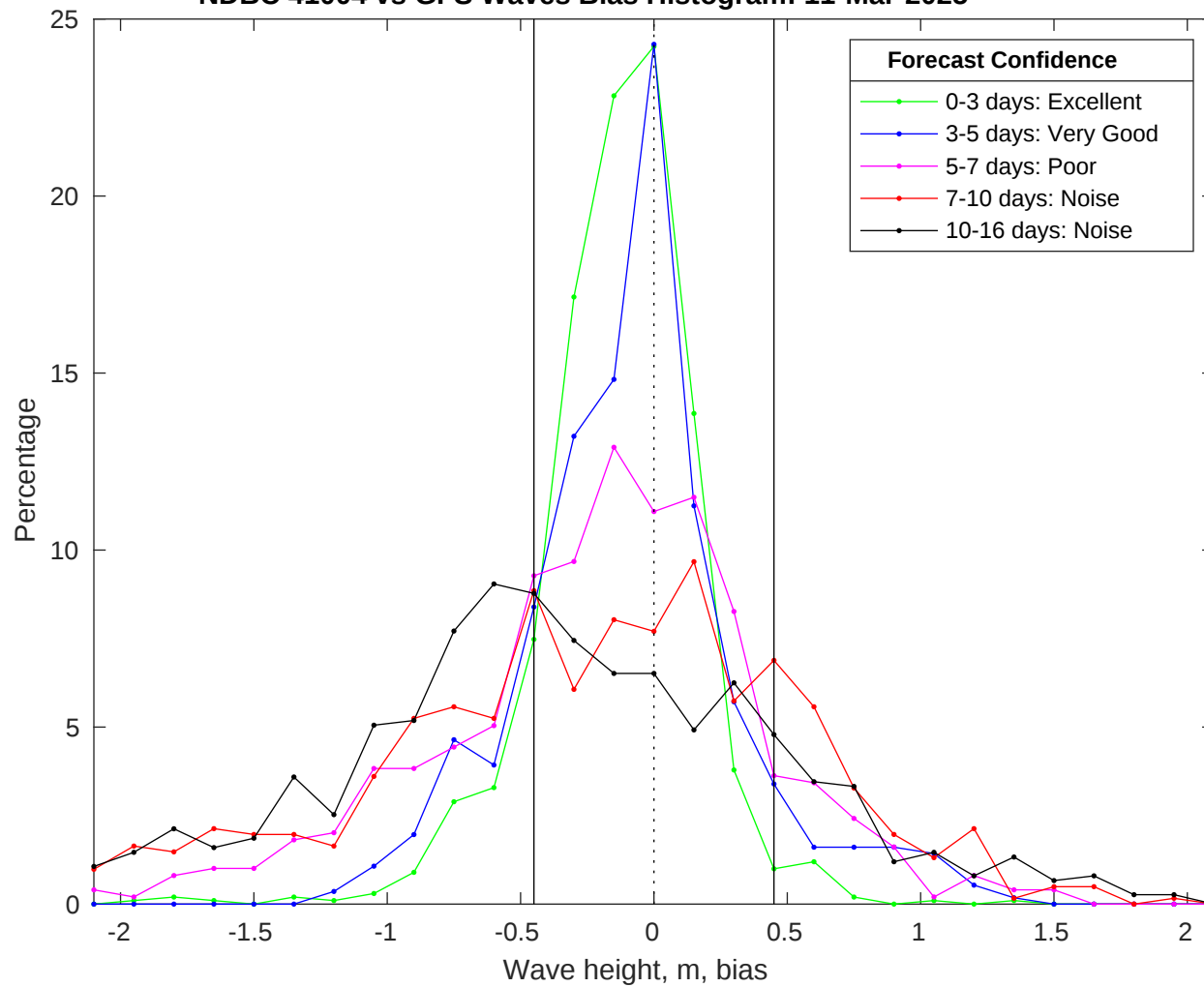
NDBC 41004 vs GFS Waves Bias Histogram: 11-Mar-2025
