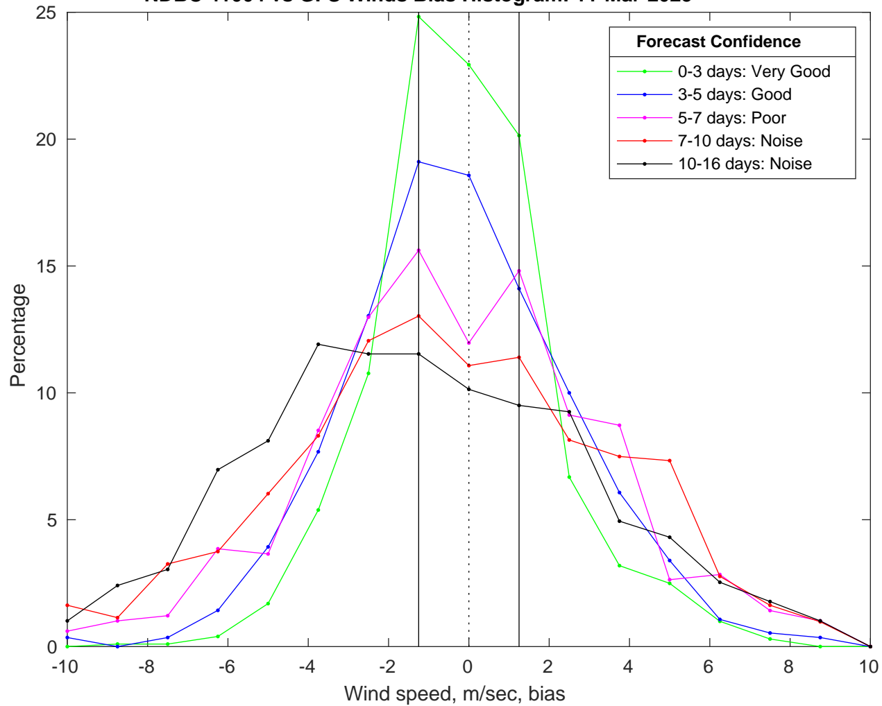
NDBC 41004 vs GFS Winds Bias Histogram: 11-Mar-2025
