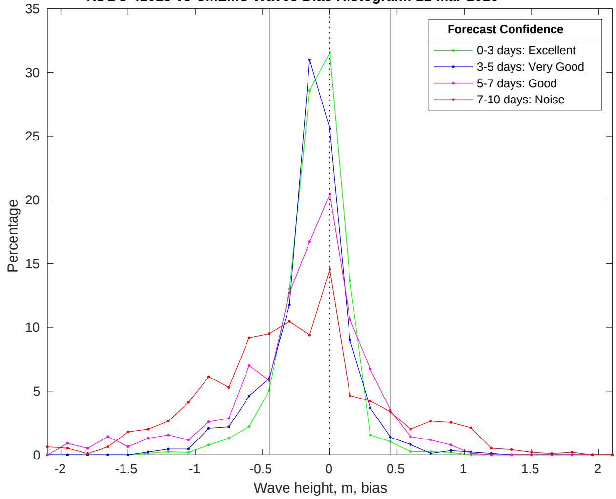
NDBC 41013 vs CMEMS Waves Bias Histogram: 11-Mar-2025
