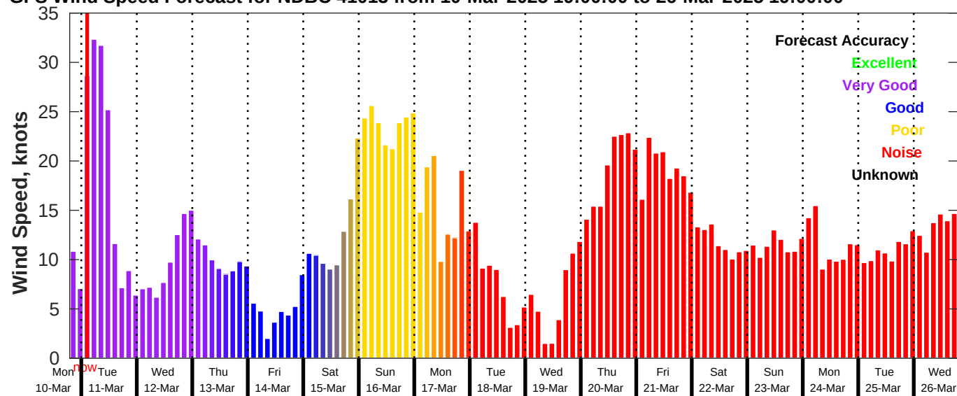
GFS Wind Speed Forecast for NDBC 41013 from 10-Mar-2025 19:00:00 to 26-Mar-2025 19:00:00
